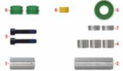
KISA PERNO 37,70x76 UZUN PERNO 38x63/118 MAXX22 T - SCHMITZ DORSE
